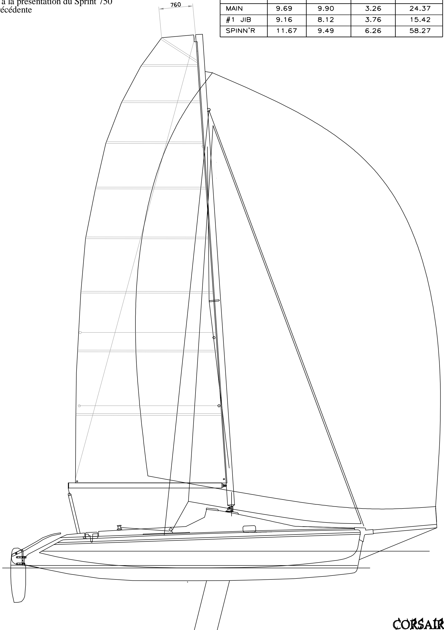
SPRINT 750 SAILPLAN JANUARY 2005
